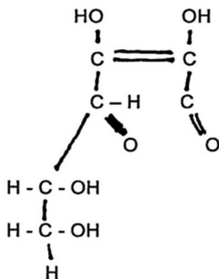
Ascorbic Acid
