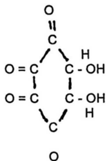
Rhodizonic Acid
