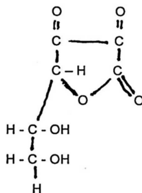
Dehydroascorbic Acid
