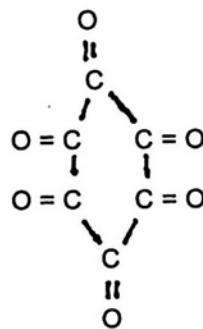
Triquinoyl
