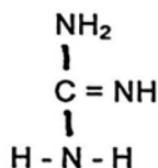
Guanidine
