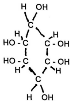
Inosital
