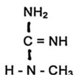
Methylguanidine
